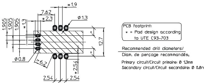
Figure 9: PCB footprint
